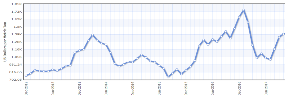
Palm Kernel Oil Monthly Price - US Dollars per Metric Ton
